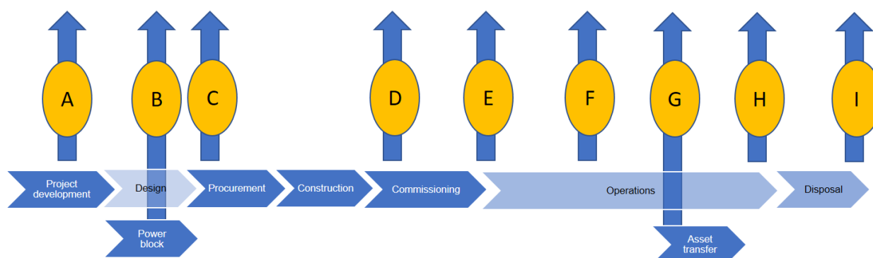
Figure 1: PV power plant lifecycle milestones-phases indicated in capital letters A through H.
